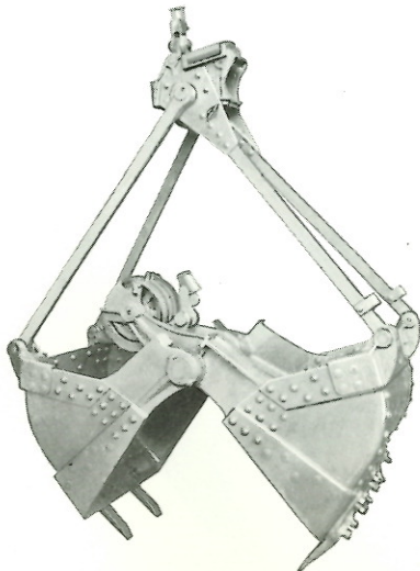
Blaw-Knox two-line lever arm type general purpose bucket. "600" Series.
